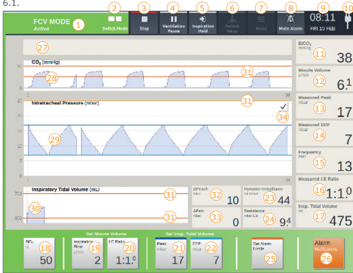
Figure 6.3. User interface aspects in FCV® Mode.
