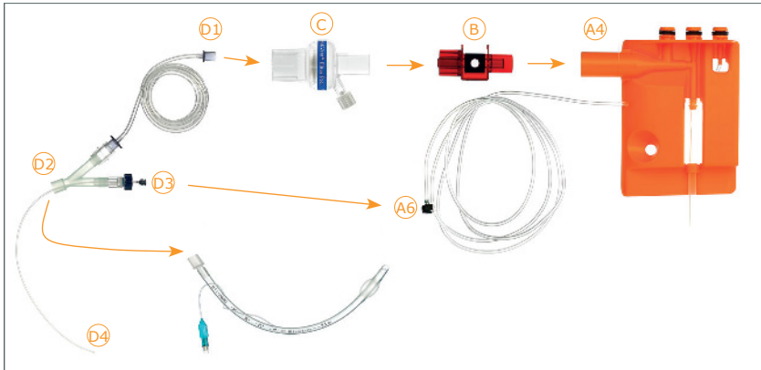
Figure 4.3. Assembly order of Airway Adapter, HME filter, Evone® Conventional Tube Adapter and additional part conventional adult endotracheal tube (example). Parts are explained in Table 2.2.
