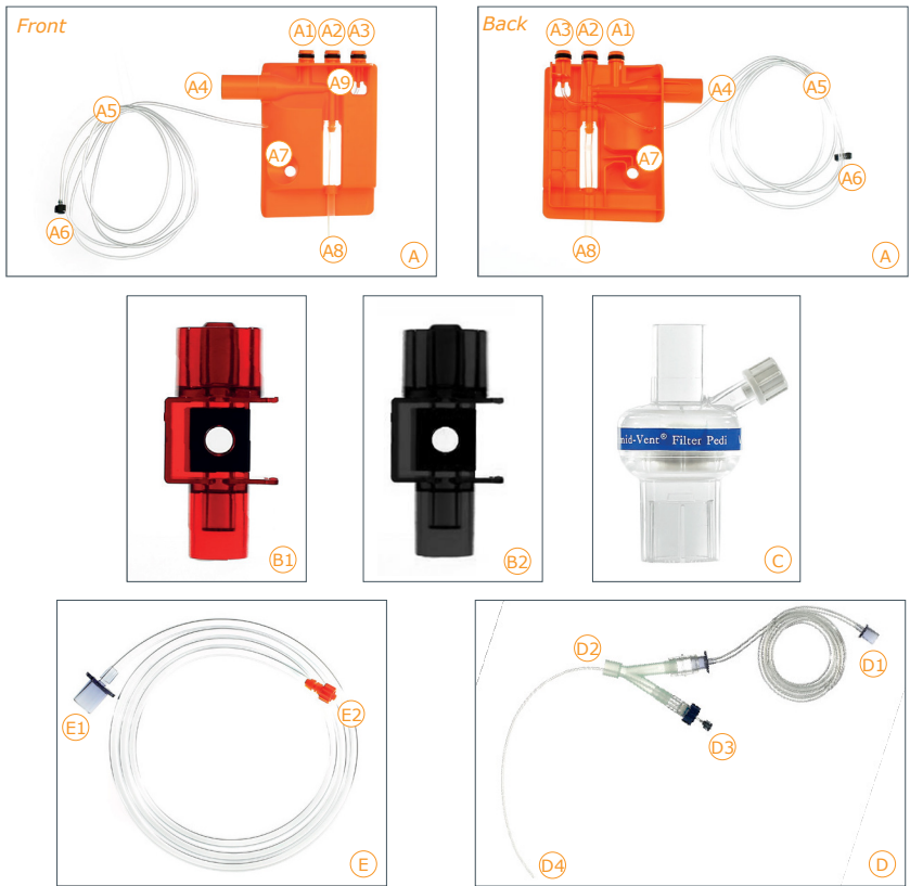
Figure 2.3. Evone® Breathing System (A-E).
