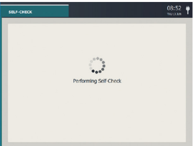
Figure 5.1. Self-Check screen.
