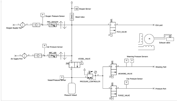
Figure 10.1. Pneumatic diagram of Evone®.
